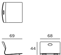
LOUNGESTUHL LOUNGE CHAIR
