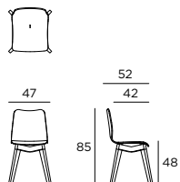
STUHL HOLZ CHAIR WOOD
