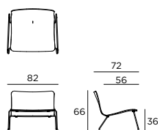
LOUNGESTUHL STAPELBAR STACKABLE LOUNGE CHAIR
